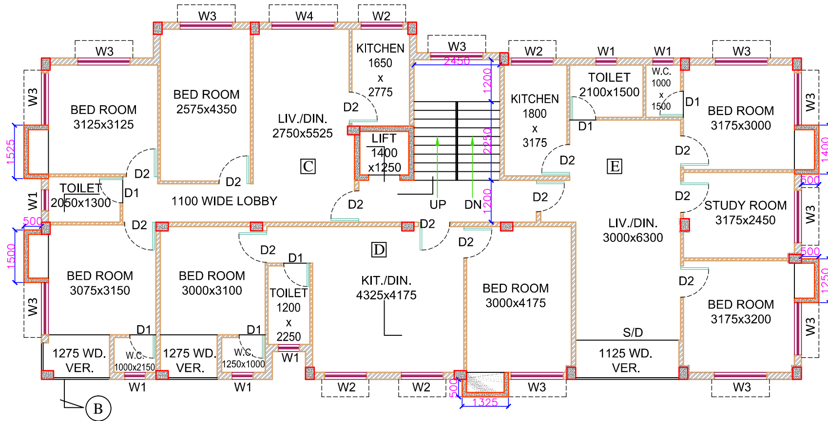
TYPICAL FLOOR PLAN (1st & 2nd) SCALE - 1 : 100
